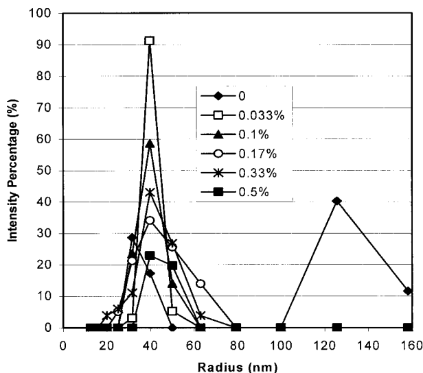
Figure 4. Size distribution functions from DLS for samples with C_s varying from 0.0 to 0.50%, and C_{lp} = 0.33 wt %.
